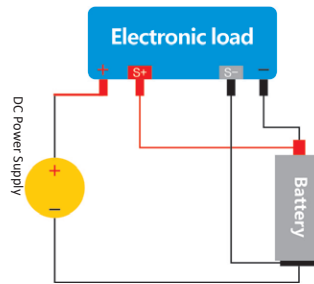
▲ Charge Wiring
